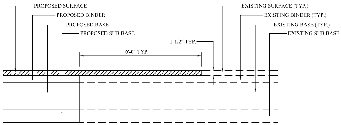
SECTION B-B
